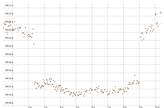
Side profile of road with hard curbs and asphalt surface captured with high precision and accuracy.
